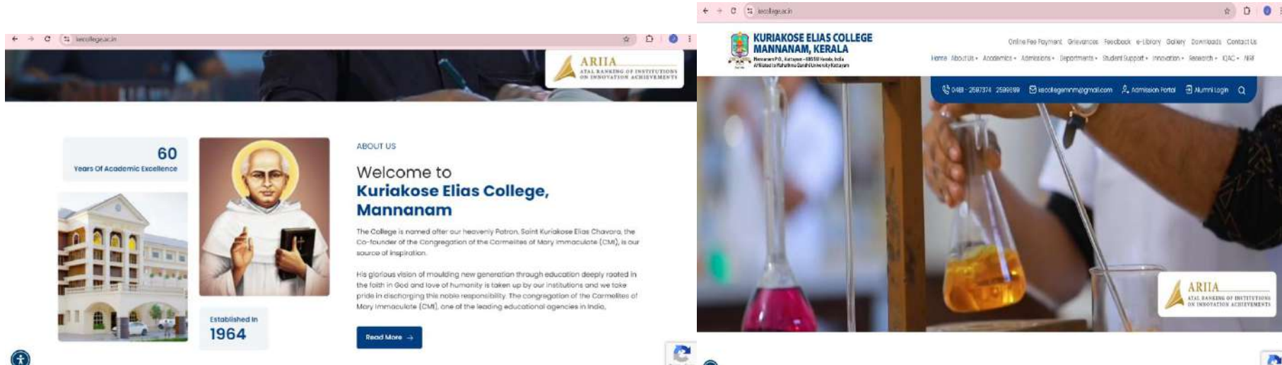
Revamped Website
