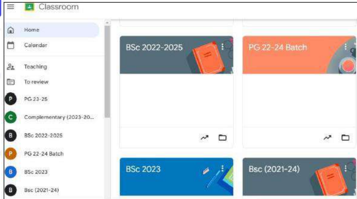
Google Classrooms
